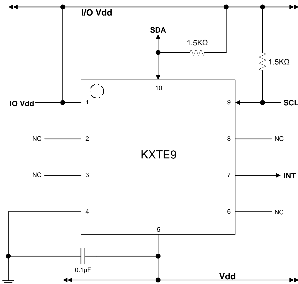
Figure 1: Application Schematic
